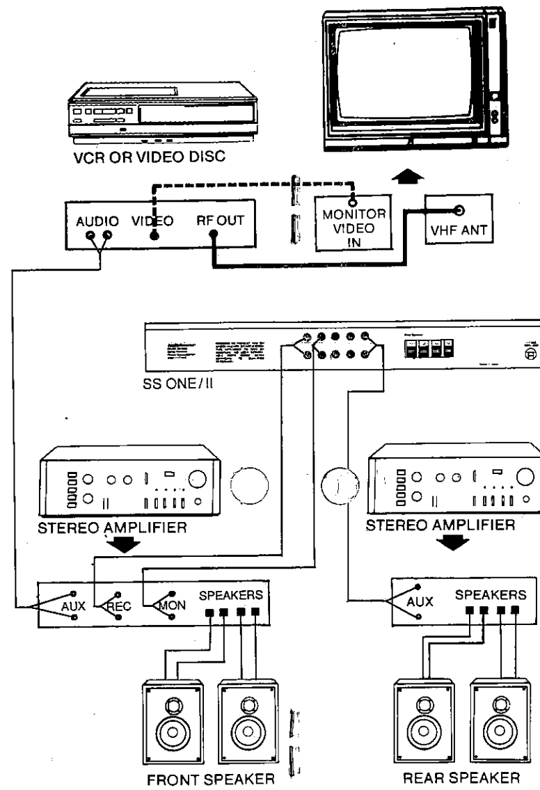
■ TV (mono sound), Stereo VCR and using two external Stereo Amplifiers for the front and rear sound field
